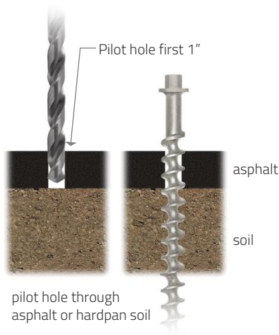
Pre drill pilot hole with impact wrench (this determines holding power). Earth Anchor can then be installed.
